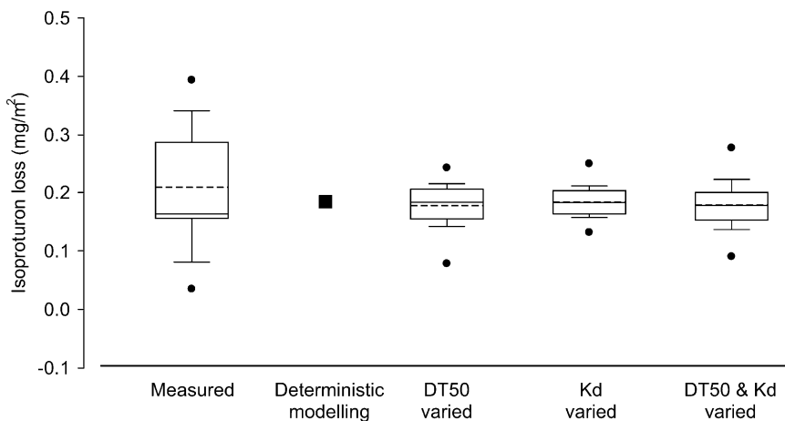
Fig. 6. Box-and-Whisker plots for measured isoproturon losses from the Hodnet lysimeters and for those simulated following variation of pesticide input parameters for MACRO (symbols as in Fig. 1; (■) isoproturon loss simulated with average parameters).
