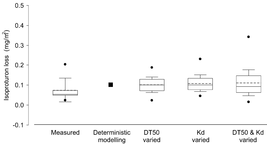
Fig. 5. Box-and-Whisker plots for measured isoproturon losses from the Wick lysimeters and for those simulated following variation of pesticide input parameters for MACRO (symbols as in Fig. 1; (■) isoproturon loss simulated with average parameters).
