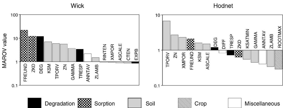
Fig. 4. MAROV indices (–) for the 15 most sensitive input parameters for MACRO for loss via leaching from the Wick and Hodnet soil of a pesticide with Koc = 100 ml g -1 and DT50 = 60 days at 8 °C. The larger the MAROV index the greater the sensitivity of MACRO to this particular parameter (from Dubus and Brown, 2002).
