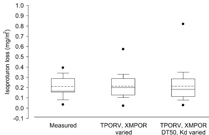
Fig. 7. Box-and-Whisker plots for measured isoproturon losses from the Hodnet lysimeters and for those simulated following variation of input parameters for MACRO (symbols as in Fig. 1).
