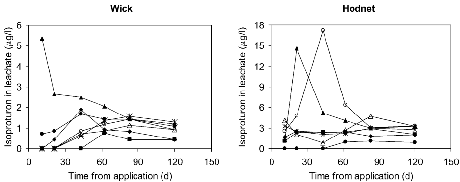
Fig. 2. Concentrations of isoproturon in leachate from the Wick and Hodnet soil lysimeters (seven replicates per soil).
